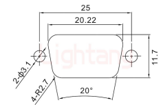
板前安装开孔 (Front Install Cutout)
