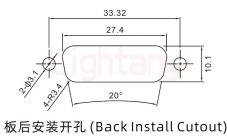
板后安装开孔 (Back Install Cutout)
